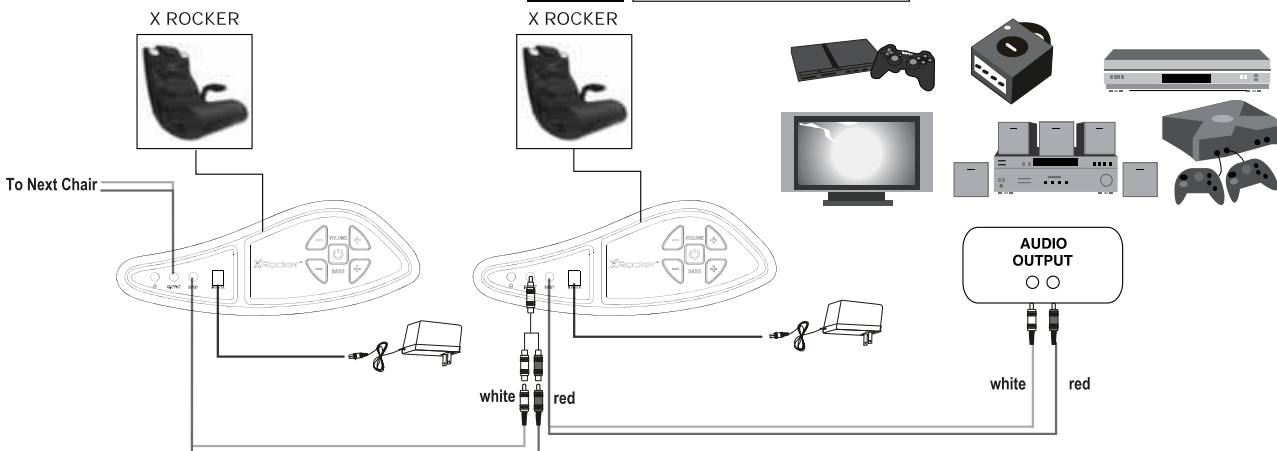
DIAGRAM 4 MULTI-USER CONNECTION
